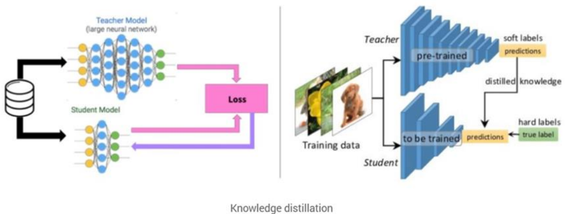
Figure : Illustration du processus de Knowledge Distillation.
